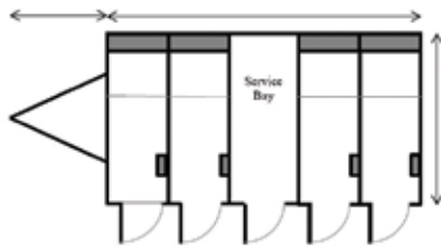
Shower 4 Bay 20ft 4" x 7ft 6" (6.2m x 2.3m)
