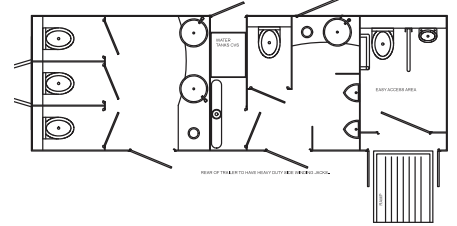
3 Ladies + 1 Gents + 2 Urinals + 1 Disabled 26ft 6" x 7ft 6" (8.2m x 2.3m)
