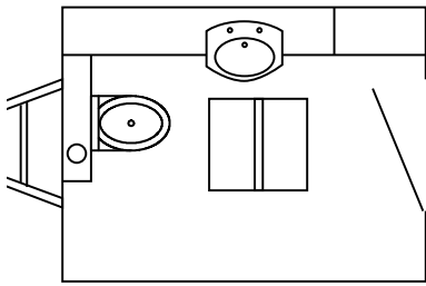
Disabled Toilet Trailer w/Ramp 8ft x 6ft (2.41m x 1.8m)
