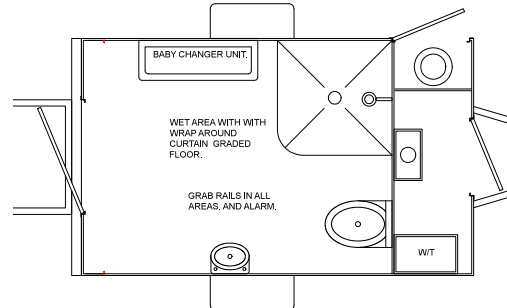
Wet Room 13ft 6" x 6ft (4.2m x 1.8m)
