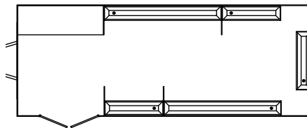
Gents 22 Man Waterless Urinal 23ft 6" x 7ft 6" (7.2m x 2.3m)
