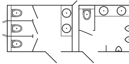
3 Ladies + 1 Gents + 3 Urinals 19ft 6" x 7ft 6" (5.9m x 2.3m)
